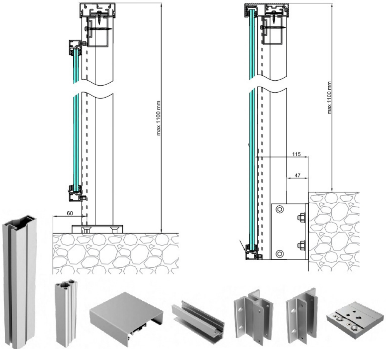
EXAMPLE TOP MOUNTING
